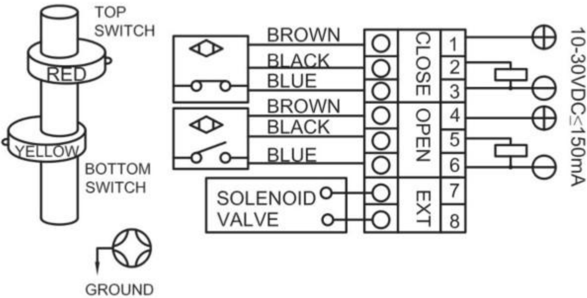
Proximity Switch (3-Wires )PNP NO APL210/DS100/DS300/DS410/DS500
