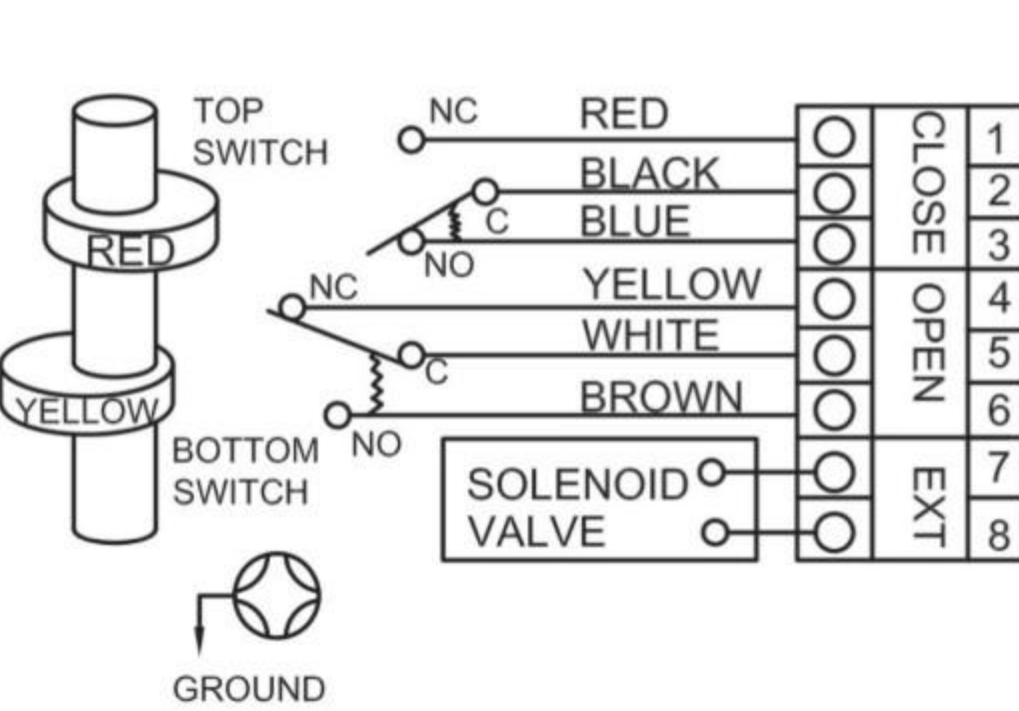
Mechanical Switch (2SPDT) APL210/ITS100/DS100/APL310/DS300/DS410/DS510
