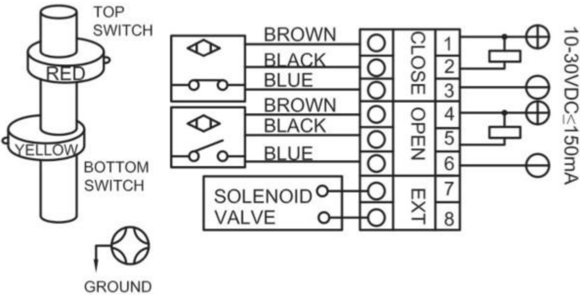
Proximity Switch (3-Wire )NPN NO APL210/DS100/DS300/DS410/DS500
