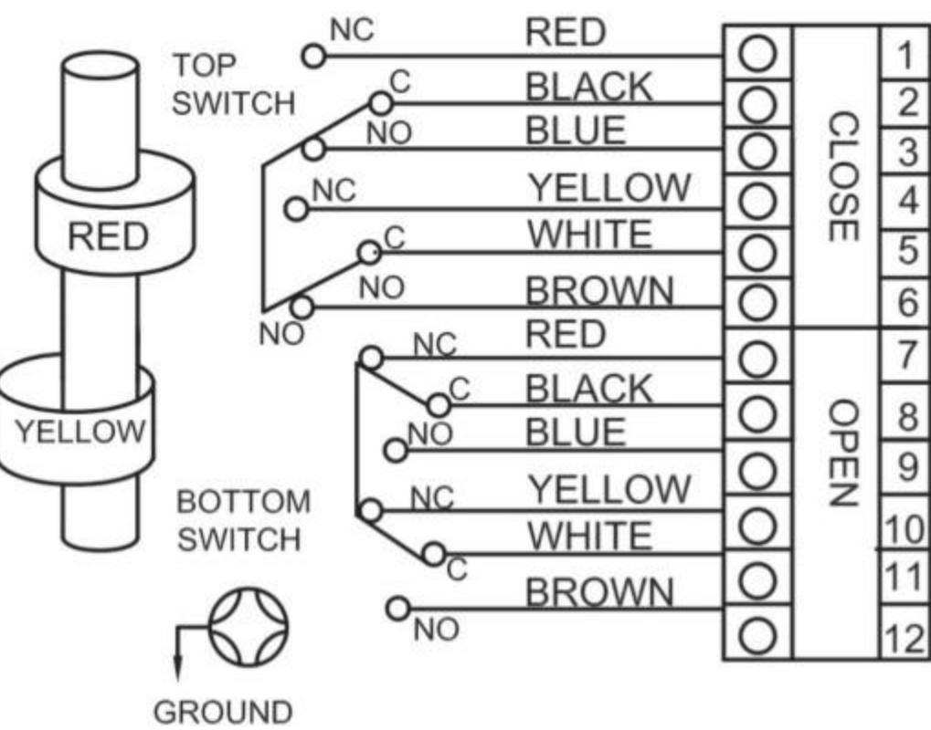
Mechanical Switch (2DPDT) DS300
