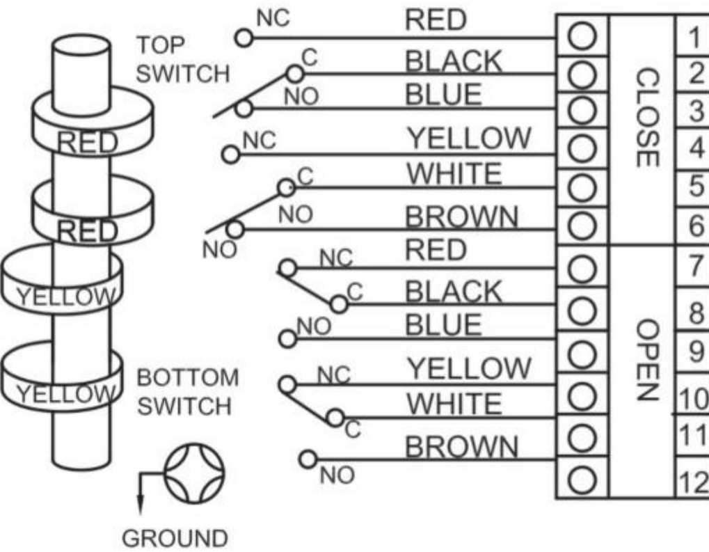
Mechanical Switch (4SPDT) DS300/APL314/ITS300
