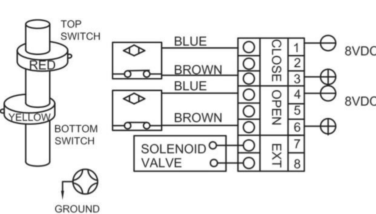
Proximity Switch(2-Wire ) APL220/DS120/DS320/DS420/DS520
