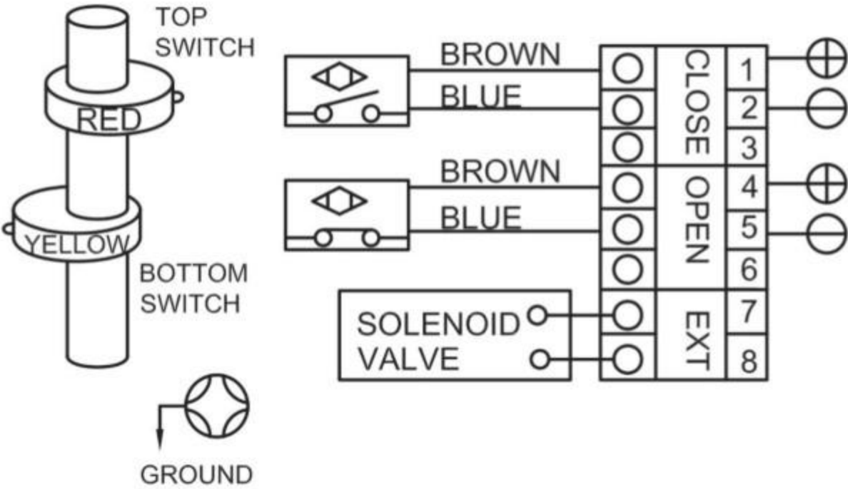
Proximity Switch (2-Wire )NC APL210/DS100/DS300/DS410/DS500
