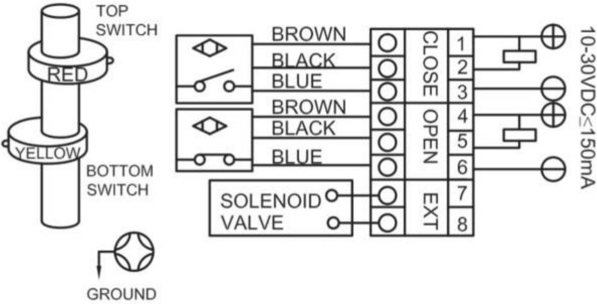
Proximity Switch (3-Wire )NPN NC APL210/DS100/DS300/DS410/DS500
