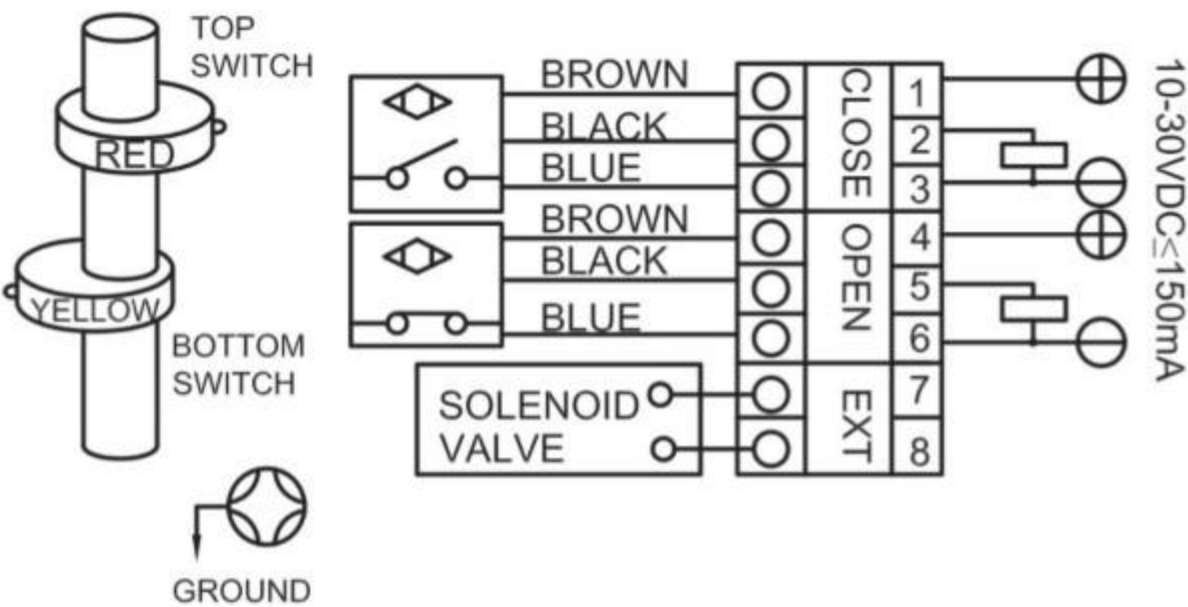
Proximity Switch (3-Wires )PNP NC APL210/DS100/DS300/DS410/DS500
